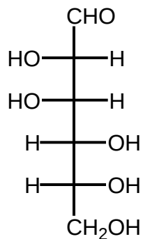
D-Mannose
