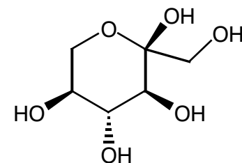
L-Sorbose
