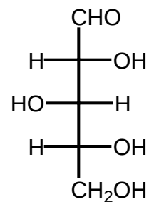
D-Xylose
