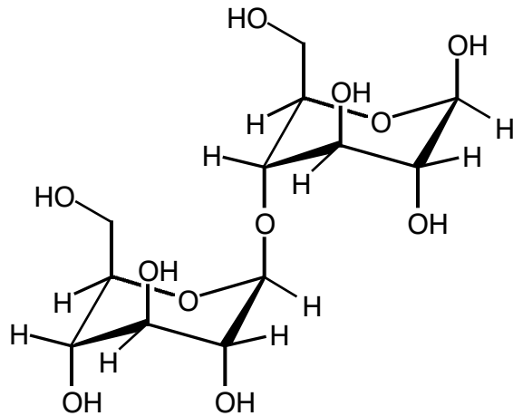
D-Cellobiose
