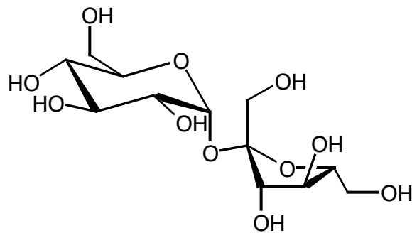
Sucrose
