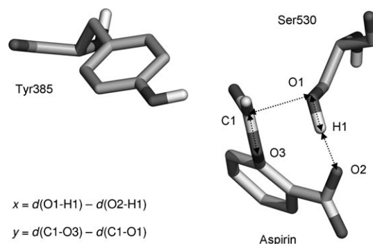
Figure 4. Definition of reaction coordinates x and y .
