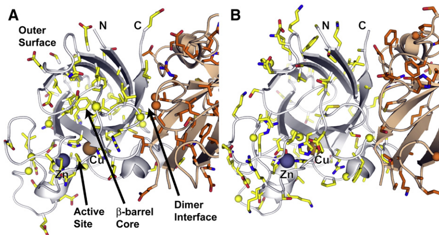
Fig. 3. Distribution of ALS mutations within the HsSOD Structure. (A) SOD residues known to be mutated in ALS patients, shown with colored side chains and spheres for glycine C \alpha atoms. One subunit is yellow, the other orange. The majority of the \beta -barrel core and edge residues, and the dimer interface residues are ALS SOD mutation sites. These residues are important for maintaining \beta -barrel stability and quaternary structure. Many outer surface residues that are mutated in ALS patients contain side chain oxygen atoms potentially important for maintaining surface electrostatic potential or for stabilizing hydrogen bonding and salt-bridge interactions. (B) SOD residues not implicated in ALS, colored and shown from the same view as in (A). The active site (lower left) and the outer surface contain many residues not linked to ALS.
