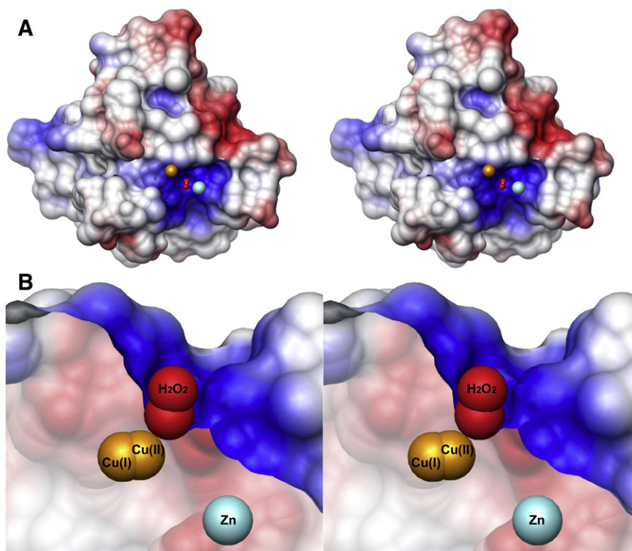
Fig. 2. (A) Electrostatic potential mapped onto the Alvinella pompejana surface from the ApSOD- \text{H}_2\text{O}_2 complex crystal structure. Electrostatic potential (blue positive, red negative) shows active site electrostatic attraction for superoxide anion. The \text{H}_2\text{O}_2 molecule (red spheres) occupies the position of the substrate/intermediate/product of the reaction. The spheres representing reduced copper (left) and zinc (right) are brought forward to show their relative positions. (B) Sliced version of the surface. From this view, the steric restrictions on the substrate/intermediate/product are readily recognized. Within the crystals, the copper ions (gold) were found in both the oxidized and reduced forms and show the short distance required for copper ion movement during SOD catalysis.
