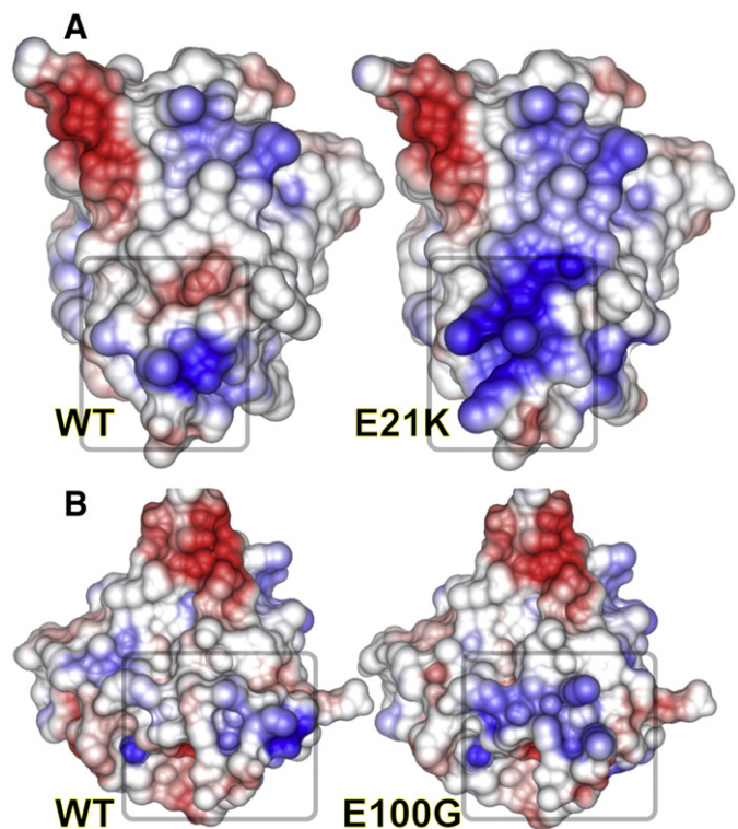
Fig. 5. Effects of single-point mutations in HsSOD on electrostatic potential. Electrostatic potential was mapped onto the surfaces of wild-type (left) vs. mutant (right) HsSOD models for the E21K and E100G HsSOD mutants. Loss of charge complementarity can dramatically change the electrostatic potential and reduce stability, both of which may result in aberrant SOD interactions.
