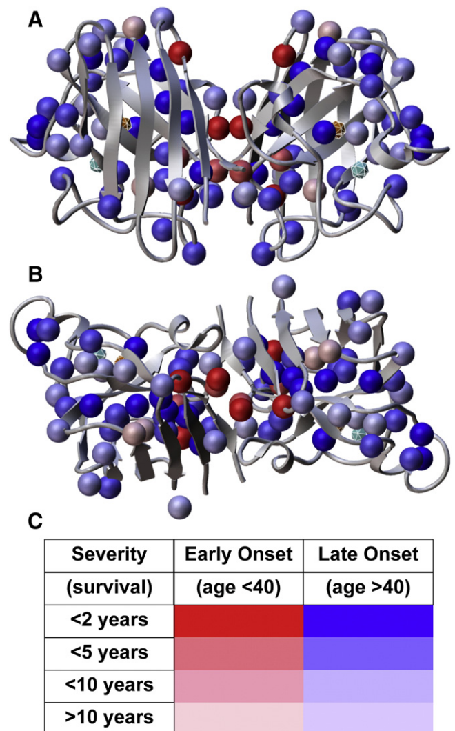
Fig. 4. Disease onset and severity mapped onto ALS mutation sites in HsSOD structure. (A) FALS mutation sites (spheres) are found throughout the SOD sequence at sites expected to reduce the integrity of the \beta -barrel, especially the packing within the \beta -barrel core, "cork" regions, the dimer interface (center) and other framework features. (B) 90° rotation from (A) around horizontal axis. (C) Color codes for the spheres in (A) and (B) show the severity and age of onset linked to each mutation. Mutations linked to the most rapid and severe mutations are located within the dimer interface or in the \beta -barrel at positions likely to destabilize the dimer interface. The active site Cu and Zn ions are also shown as spheres within cages. Data from Wang et al. [63] were used to generate the figure.
